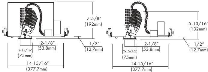
Ceiling Cut-out : SQ.2-7/8" (SQ.72mm)
